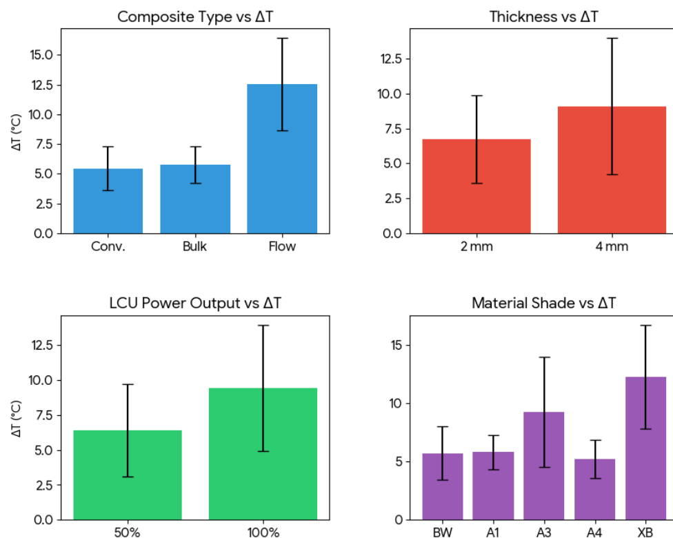
Figure 2. Effect of composite type, thickness, power output, material shade on temperature rise.
